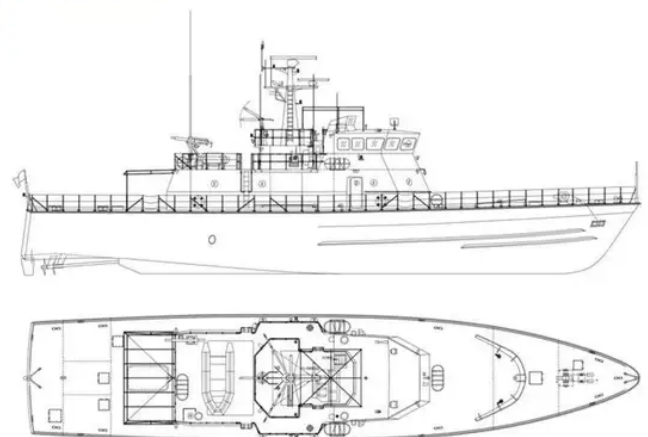
M39 PATROL BOAT
