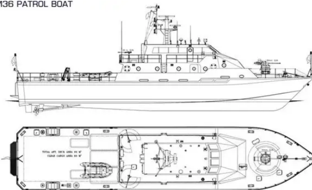
M36 PATROL BOAT
